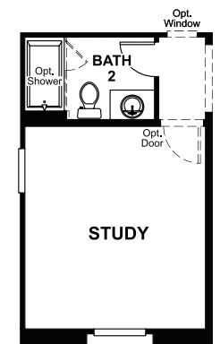
OPT. ALTERNATE ENTRANCE AT STUDY
