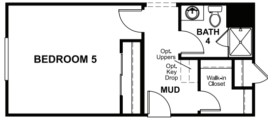
OPT. BEDROOM 5/BATH 4
