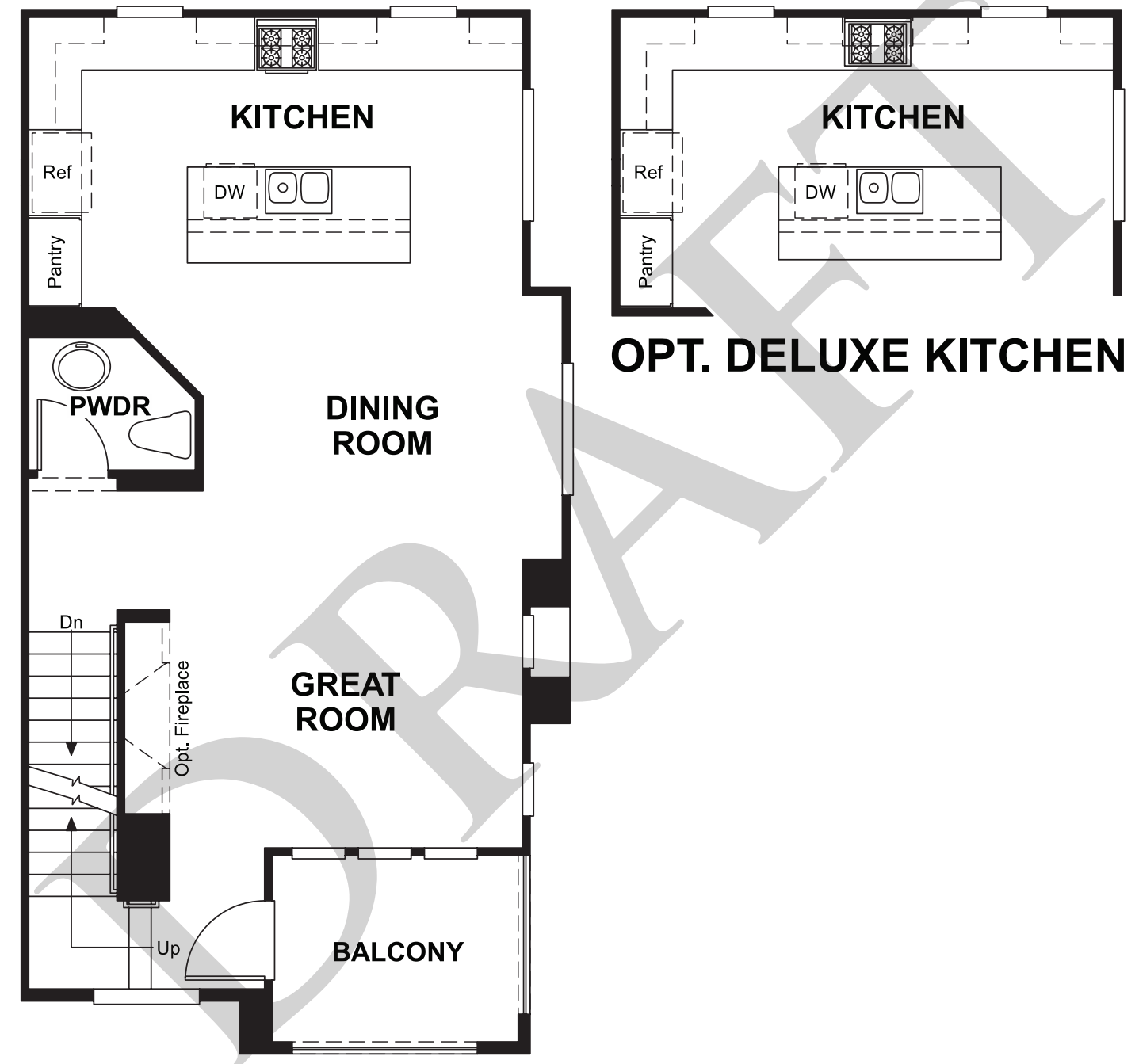
Floor Plan Main Floor
