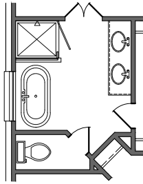
OPTIONAL TUB @ PRIMARY BATH
