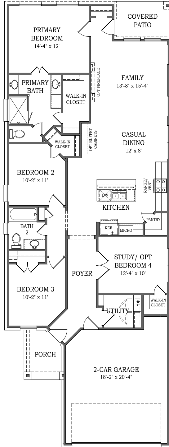
FLOOR PLAN - ELEVATION A1
