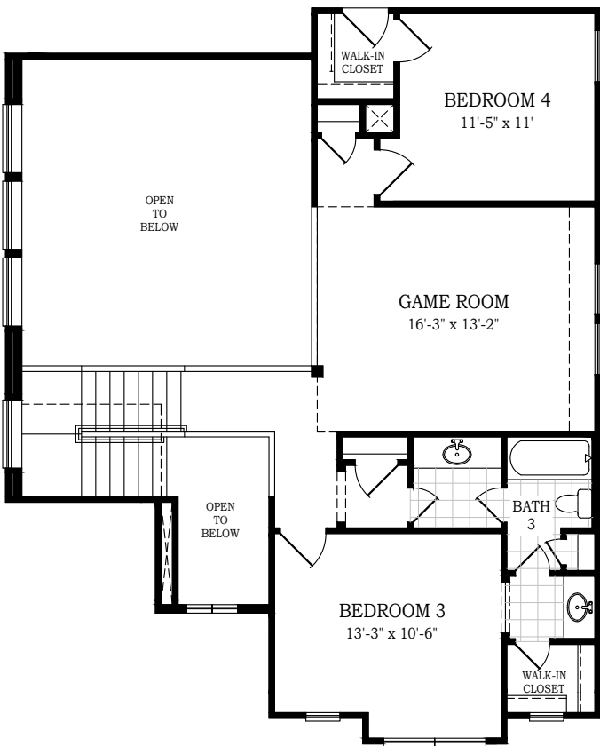
2nd Floor
