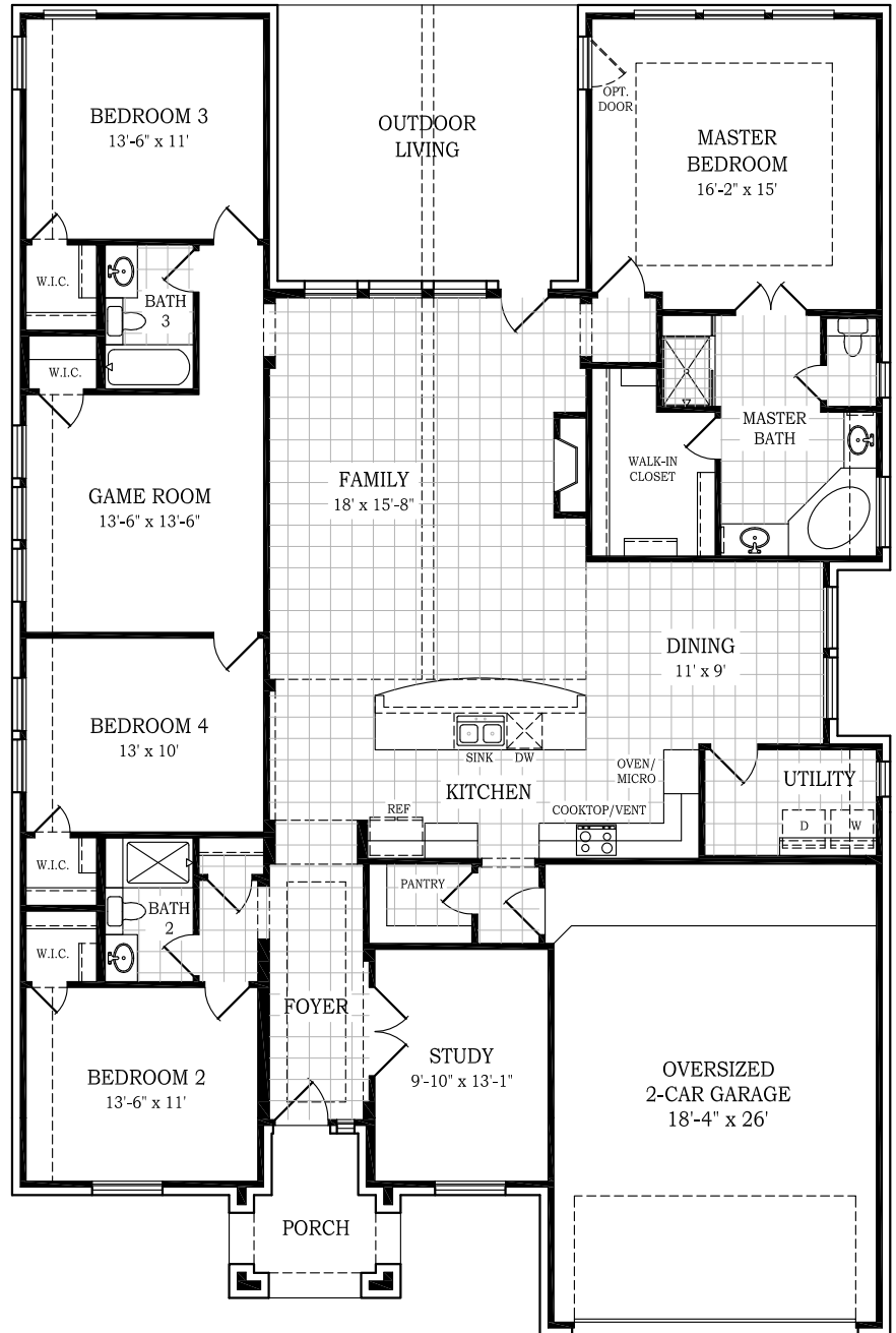
Floor Plan
