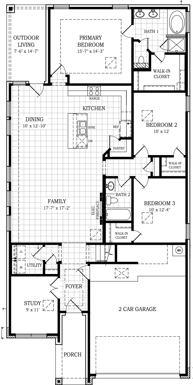
1st Floor Plan Elevation A
