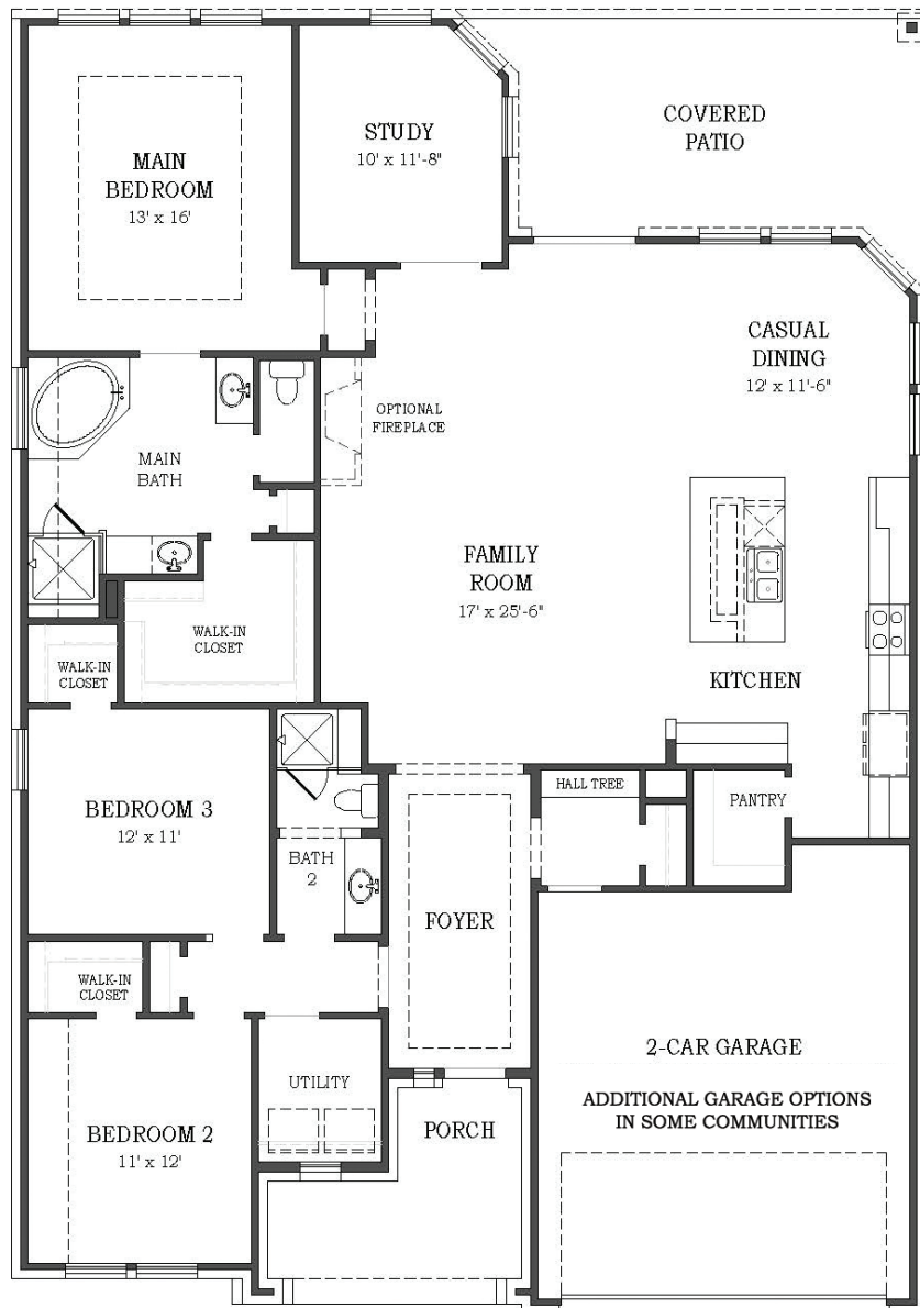
FLOOR PLAN
