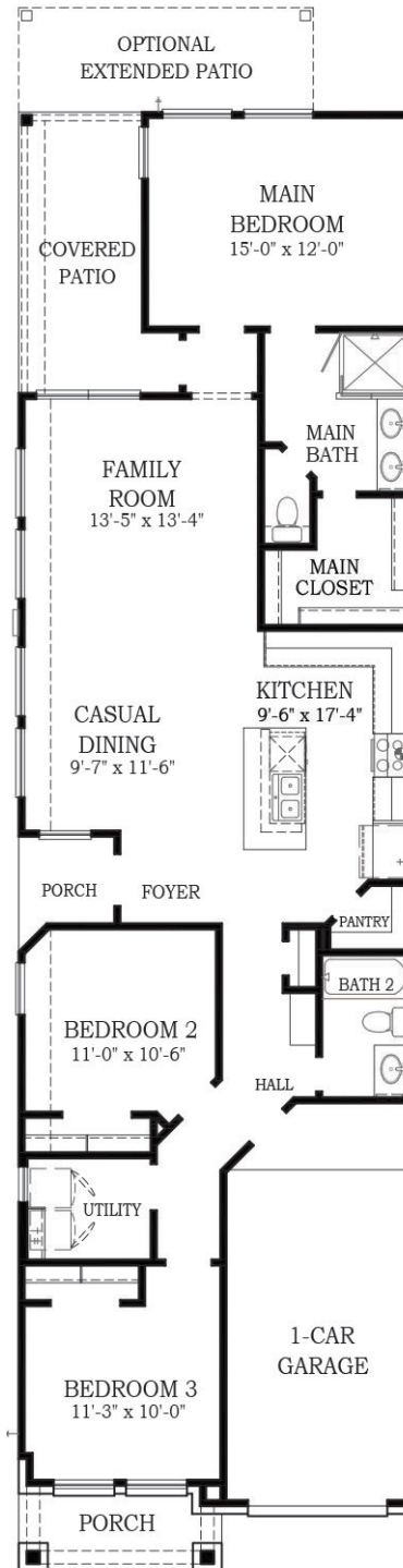
FLOOR PLAN
