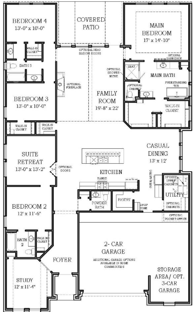
FLOOR PLAN
