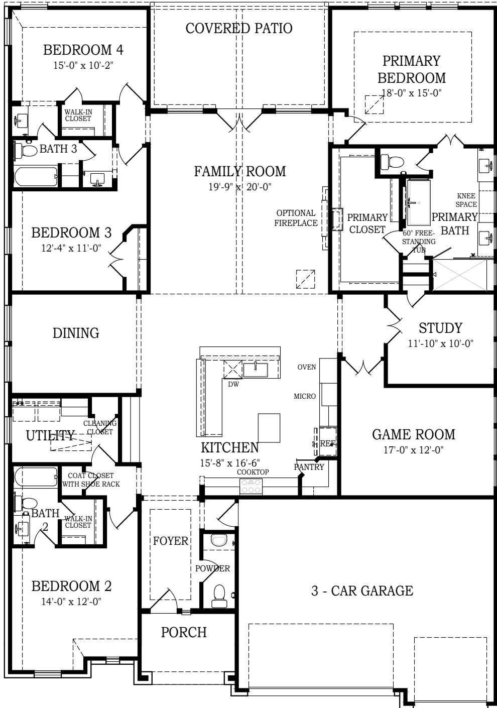
FLOOR PLAN
