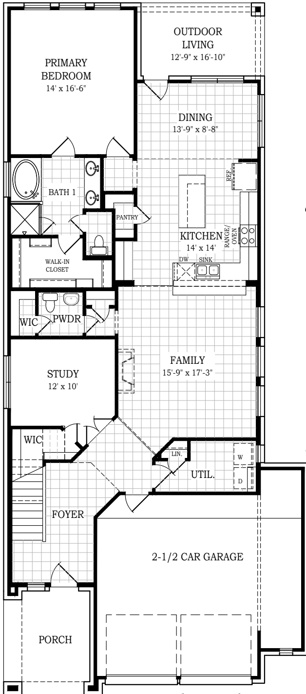
1st Floor Plan Elevation C
