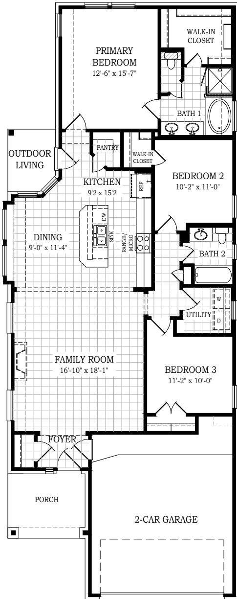
Floor Plan Elevation A
