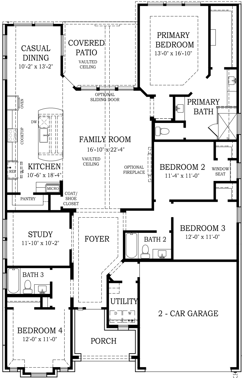
FLOOR PLAN
