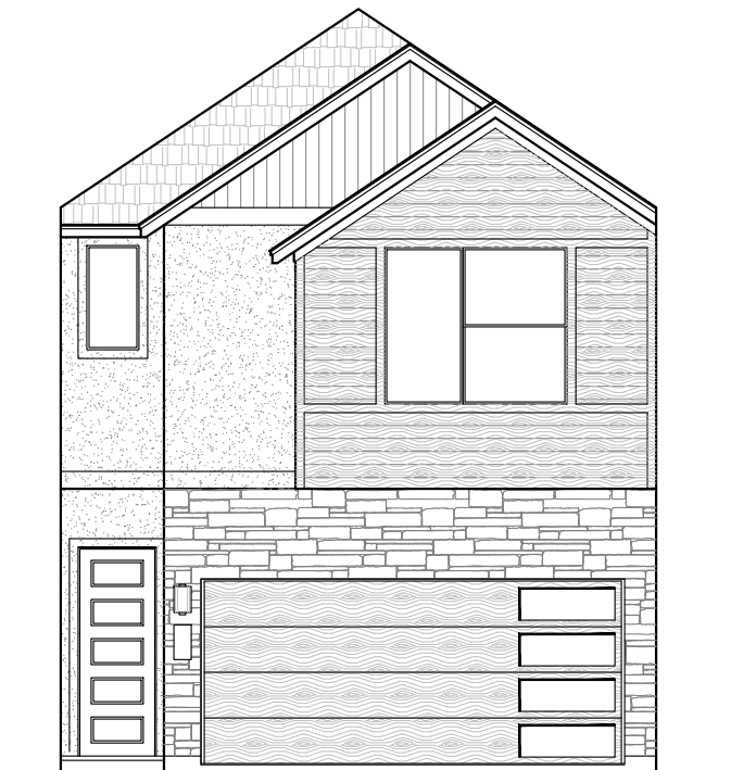
ELEVATION D
