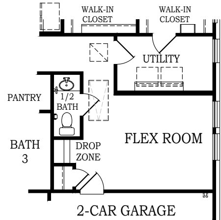
OPT. FLEX ROOM at GARAGE STORAGE
