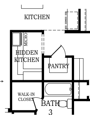
OPT. HIDDEN KITCHEN
