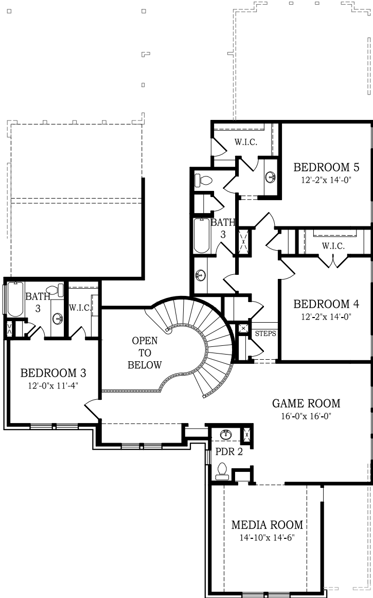
SECOND FLOOR
