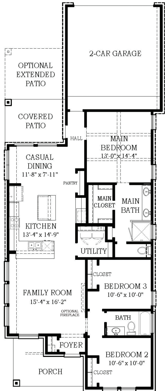
FLOOR PLAN
