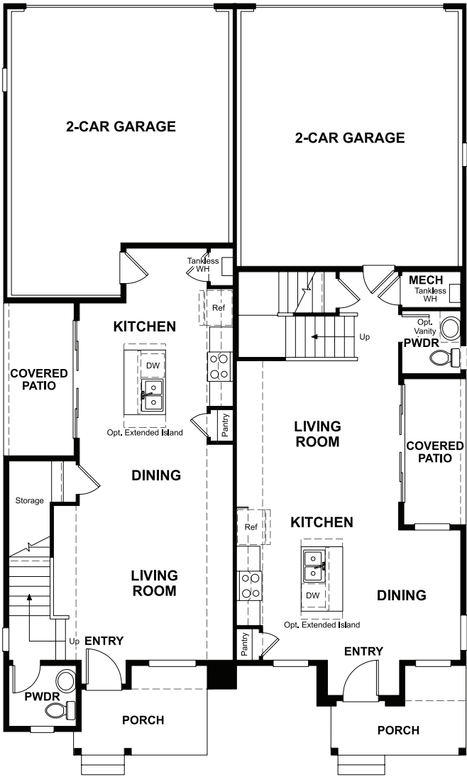
MAIN FLOOR
