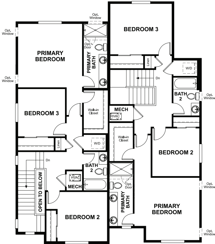
SECOND FLOOR
