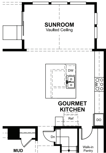
OPT. SUNROOM WITH ALTERNATE ISLAND WITH GOURMET KITCHEN
