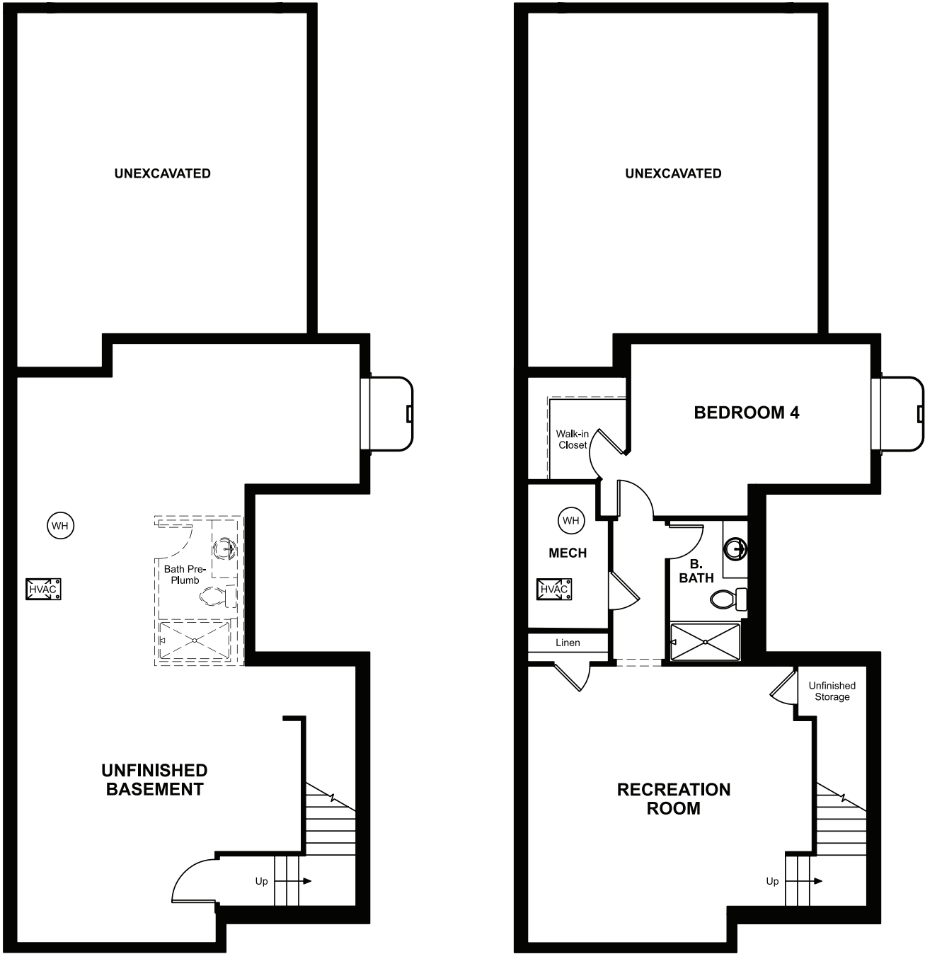
BASEMENT
