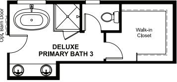
OPT. DELUXE PRIMARY BATH 3
