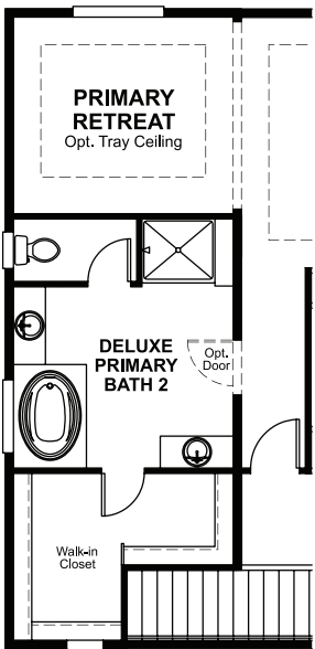
OPT. PRIMARY RETREAT/ DELUXE PRIMARY BATH 2
