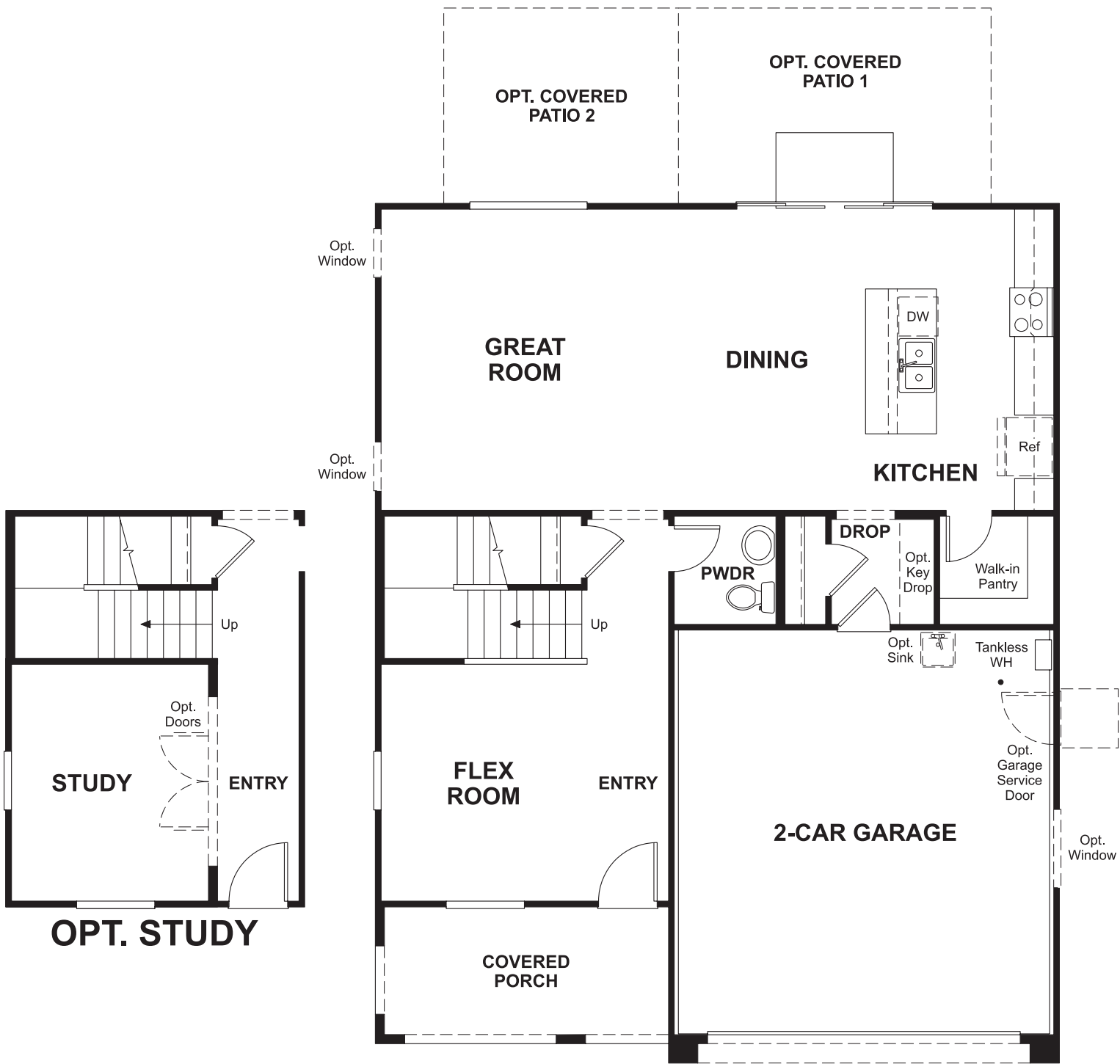
MAIN FLOOR
