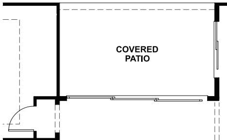
OPT. 15' MULTI-SLIDE DOORS
