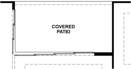
OPT. CORNER-MEET DOORS
