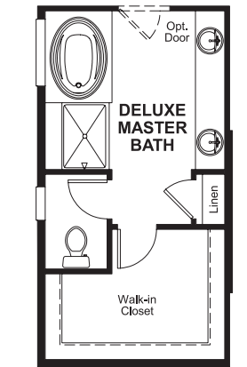
OPT. DELUXE MASTER BATH 1
