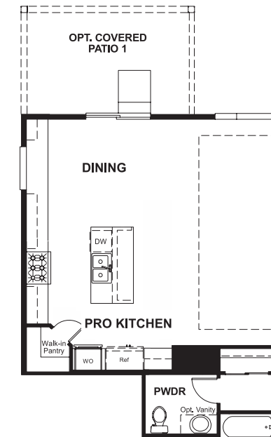
OPT. PROFESSIONAL KITCHEN W/ POWDER BATH
