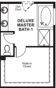
OPT. DELUXE MASTER BATH 1
