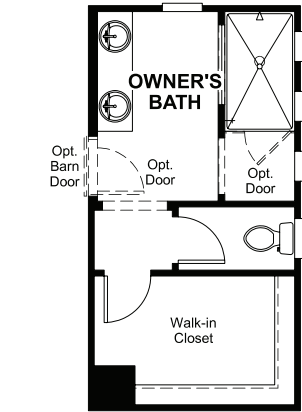
OPT. OWNER'S BATH W/ WALK-IN SHOWER
