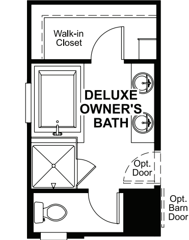
OPT. DELUXE OWNER'S BATH
