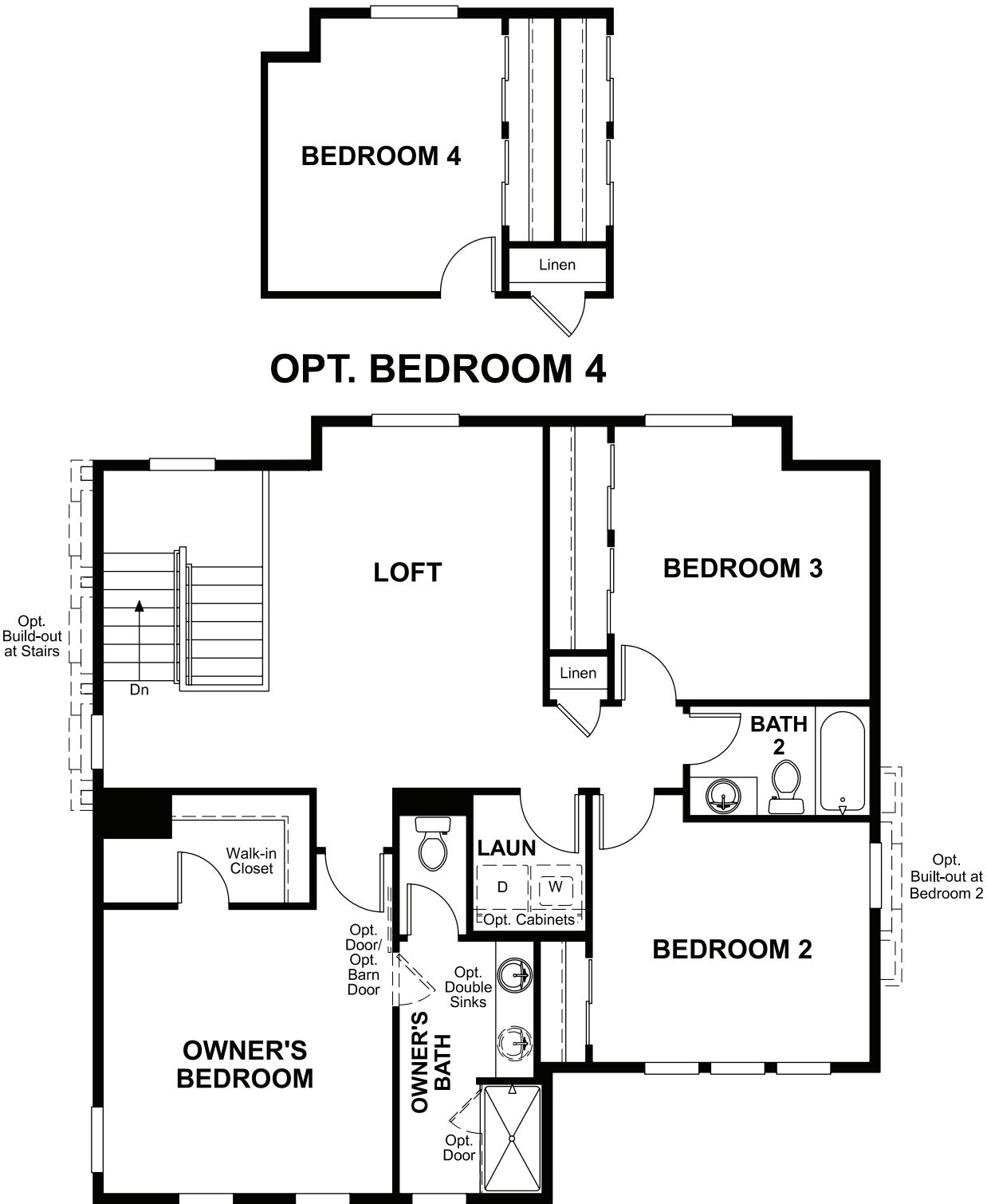
SECOND FLOOR
