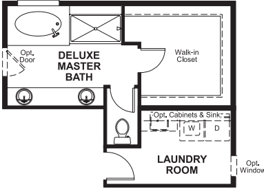
OPT. DELUXE MASTER BATH
