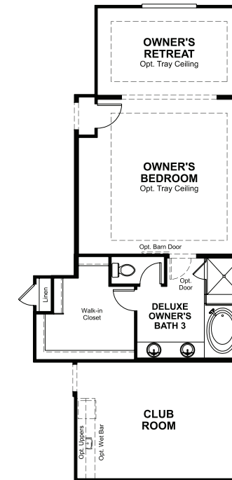
OPT. DELUXE OWNER'S BATH #3 AT OWNER'S RETREAT/CLUB ROOM
