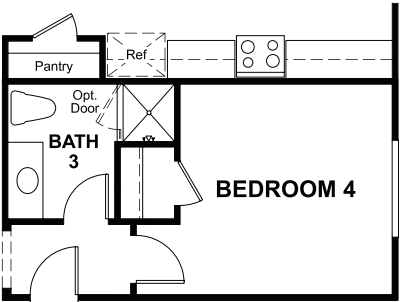
OPT. BED 4/BATH 3
