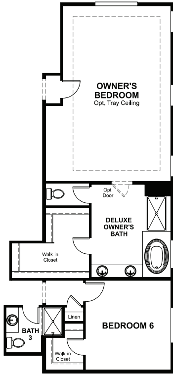
OPT. BED 6/BATH 3
