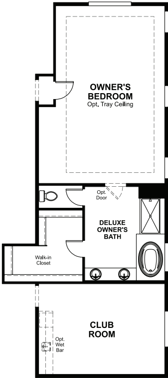
OPT. OWNER'S RETREAT/CLUBROOM
