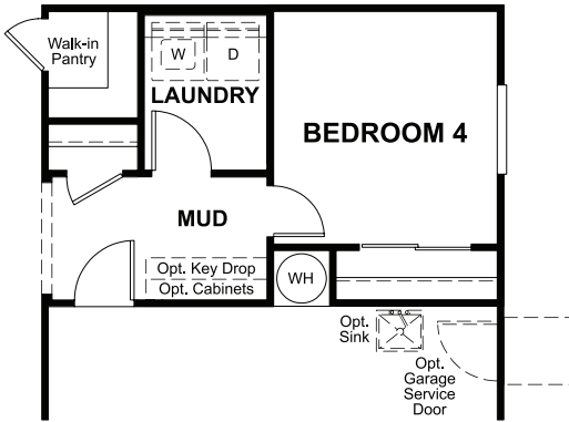
OPT. BEDROOM 4 & 2-CAR GARAGE
