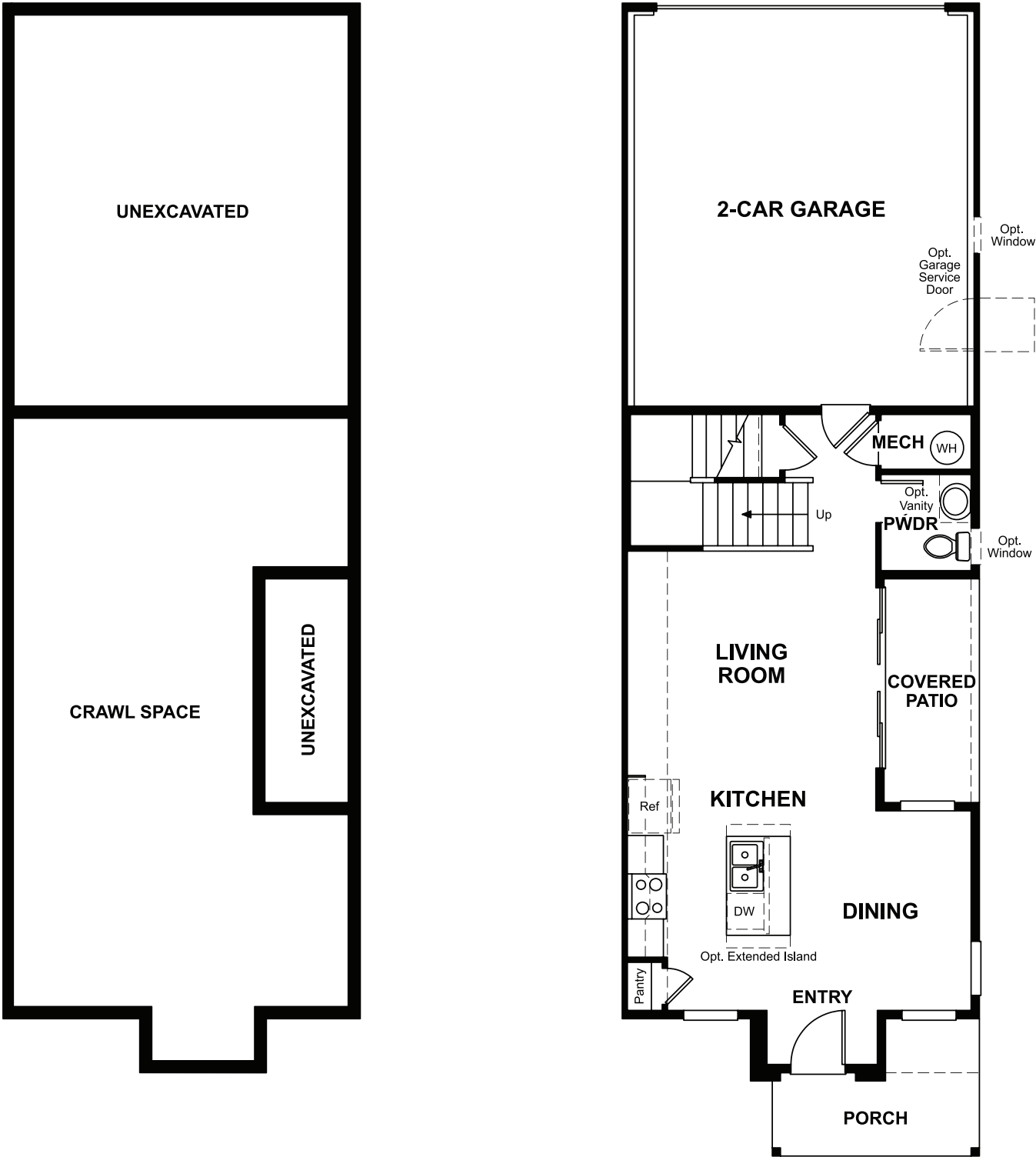
CRAWL SPACE & MAIN FLOOR
