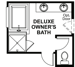
OPT. DELUXE OWNER'S BATH
