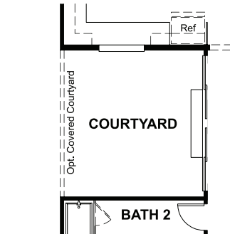
OPT. 12' CENTER-MEET DOOR AT COURTYARD
