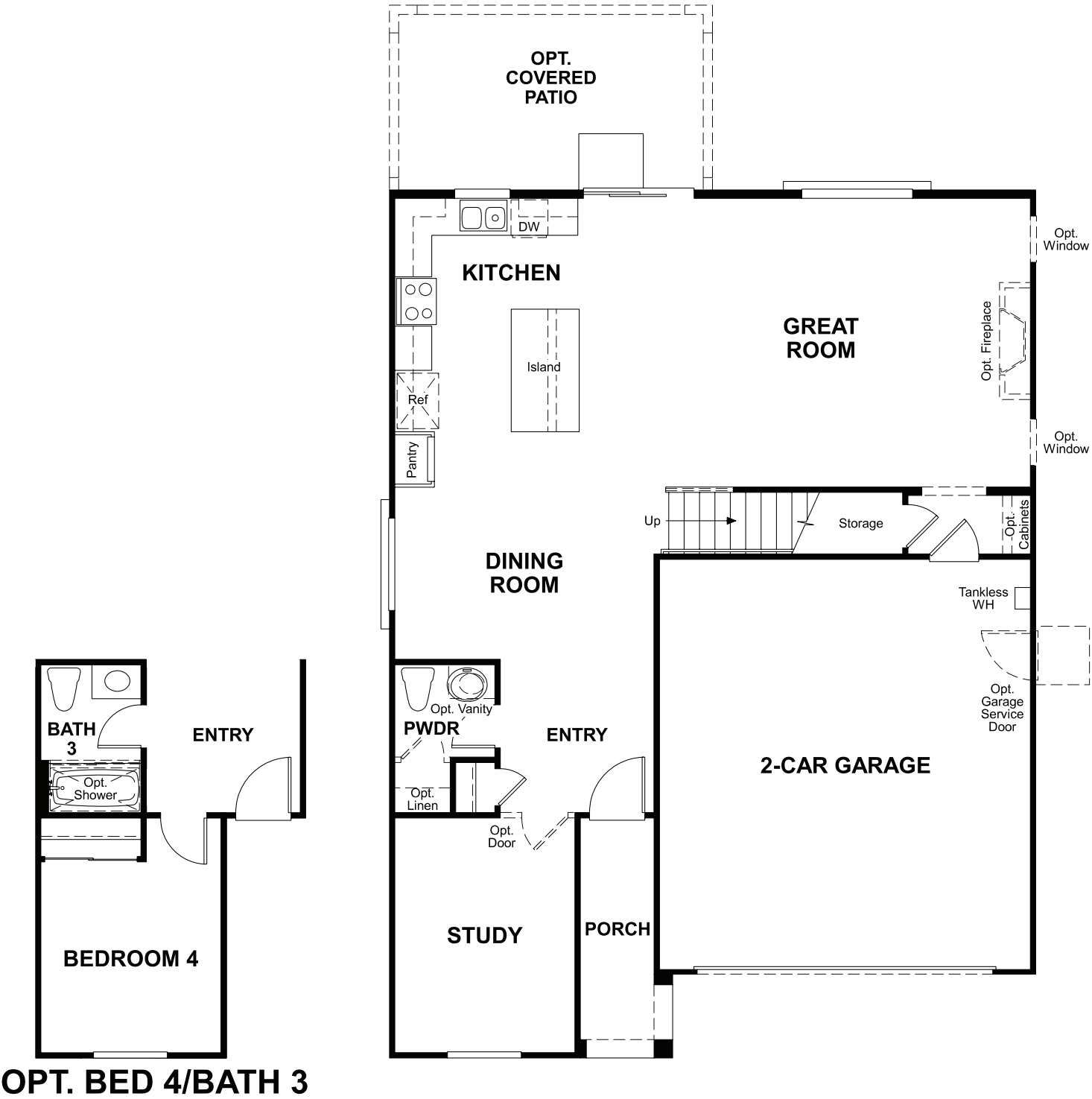
MAIN FLOOR
