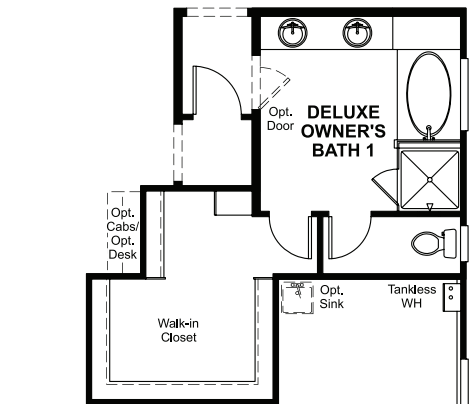
OPT. DELUXE OWNER'S BATH #1
