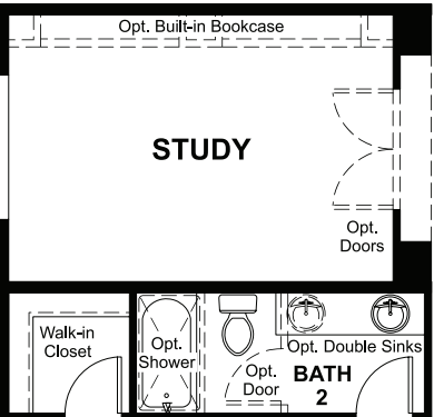
OPT. STUDY
